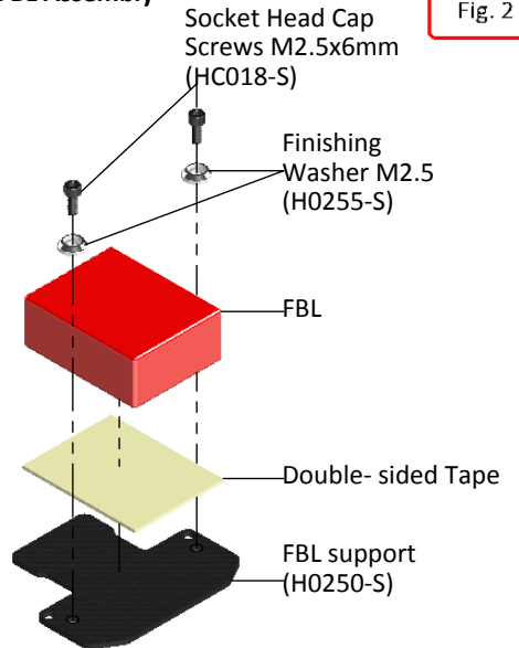
FBL Assembly
