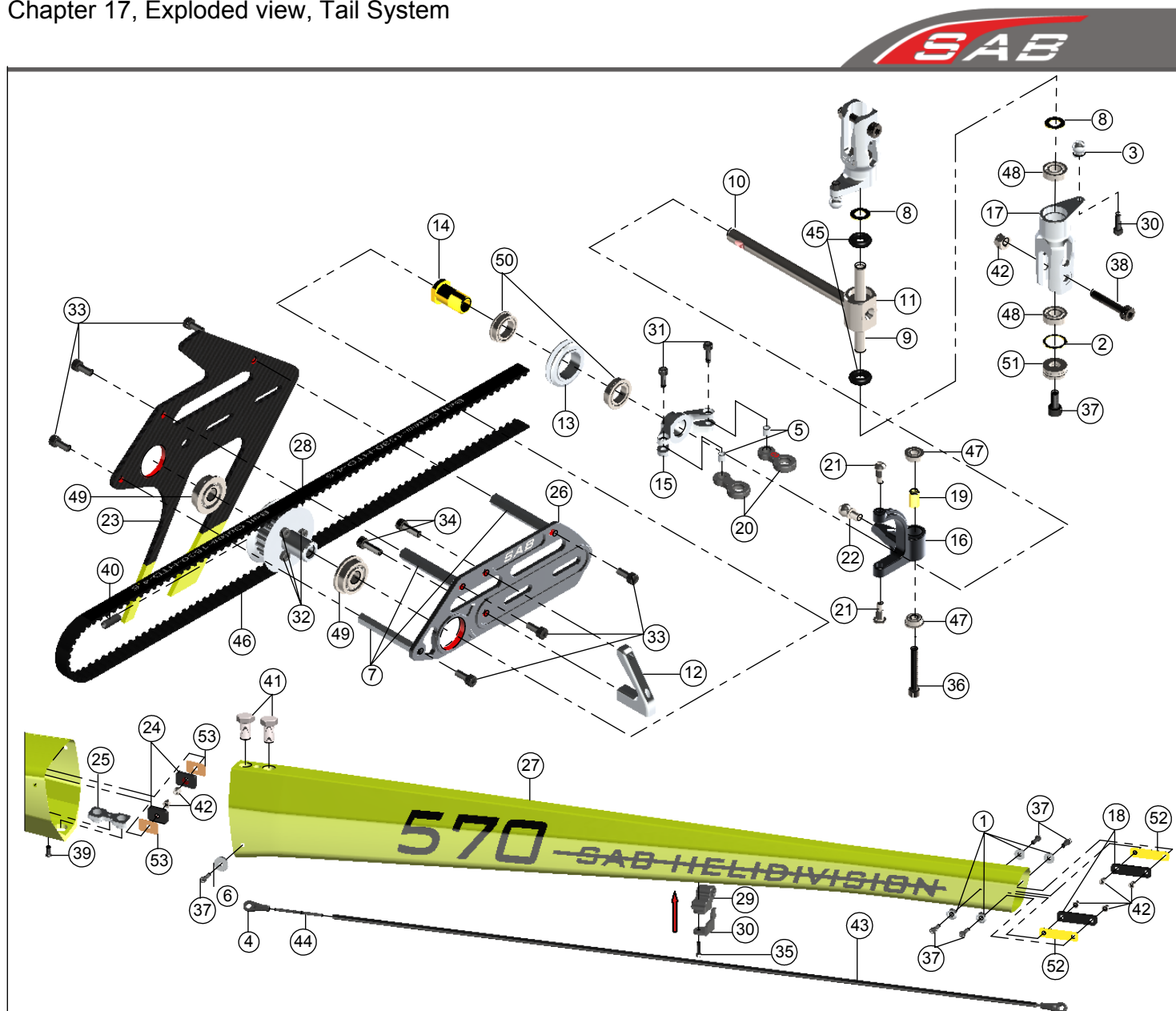
TAIL SYSTEM
